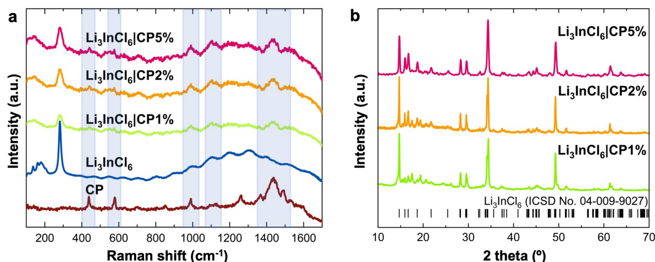
Figure 2. (a) Raman spectra of the \text{Li}_3\text{InCl}_6 |CPX composites at various wt% of the CP, as-synthesized \text{Li}_3\text{InCl}_6 and CP. The shaded regions highlighted in (a) are characteristic bands for the CP component. (b) PXRD patterns of the \text{Li}_3\text{InCl}_6 |CPX composites, including reference indices for the target main- \text{Li}_3\text{InCl}_6 phase.
