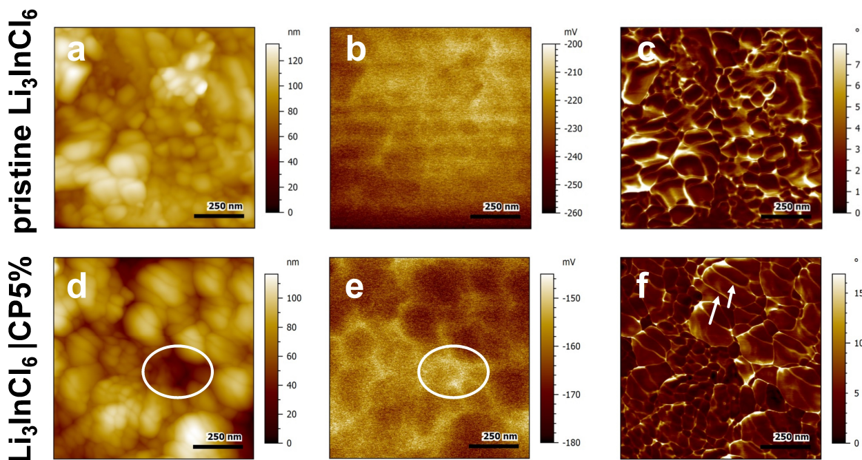
Figure 4. Exemplary topography (a and d), surface potential (b and e) and phase (c and f) images for the pristine \text{Li}_3\text{InCl}_6 sample (upper row) and the \text{Li}_3\text{InCl}_6|\text{CP5\%} composite samples (bottom row).
