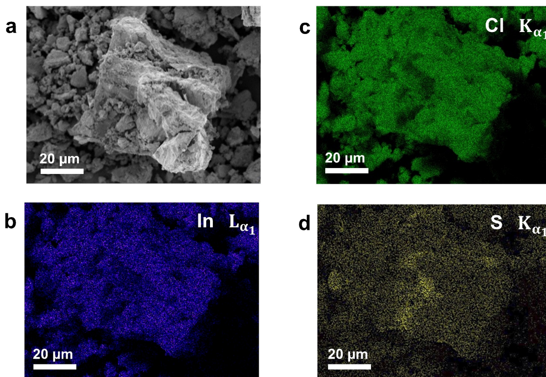
Figure 3. (a) SEM of the \text{Li}_3\text{InCl}_6|\text{CP}5\% powder particle, (b–d) EDX analysis for In, Cl and S from the image in (a).
