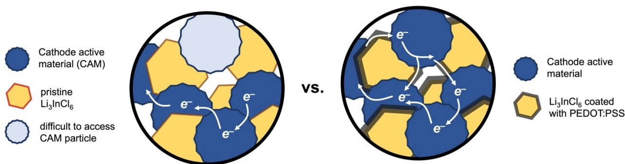
Figure 1. Schematic comparison of how the incorporation of PEDOT:PSS, an electronically conducting polymer, will improve the electronic transport as well as the utilization of the cathode active material in solid-state catholytes. In the absence of a conductive additive, cathode active material particles may be more readily isolated from participating in the cycling of the cell.
