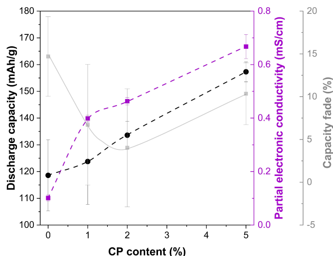
Figure 6. Correlation between the initial discharge capacities of cells, the effective electronic conductivities of the cathode composites and the capacity fade after 30 cycles at 0.1 C on the CP content.
