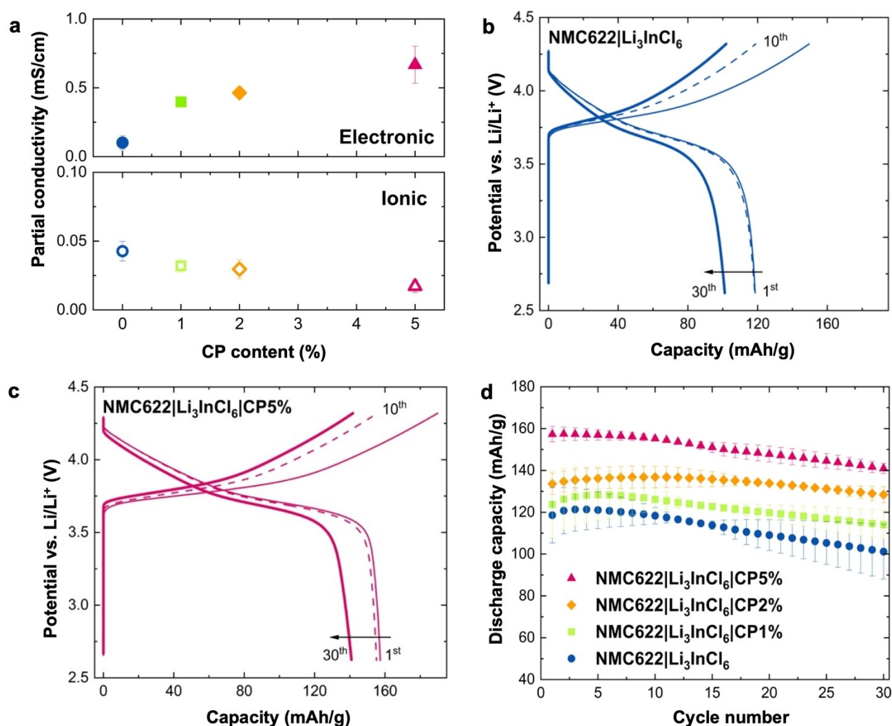
Figure 5. Evaluation of electrochemical performance of the composites. (a) Partial electronic (top) and ionic (bottom) conductivities measured via DC polarization, (b and c) charge-discharge curves of the cells (b) without and (c) with CP (5 wt% to \text{Li}_3\text{InCl}_6 ) in the catholyte composite, (d) discharge capacities up to 30 cycles for cells with different catholyte composites at 0.1 C.
